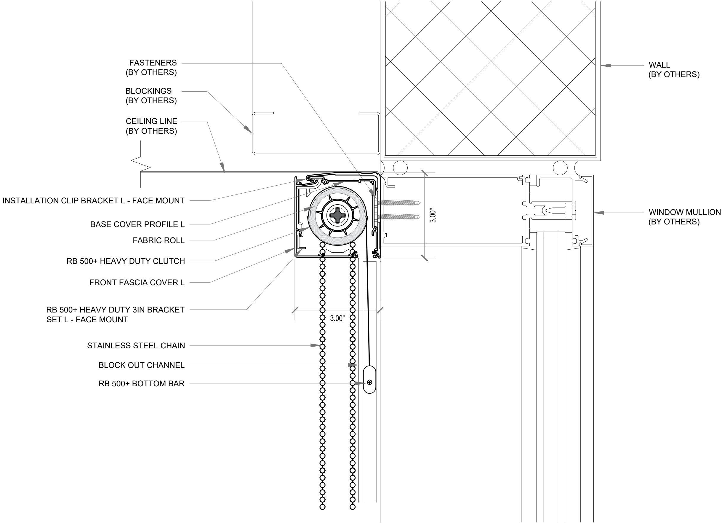
01 RB 500+ - HEAVY DUTY 3IN BRACKET SET L BLOCK OUT - SECTION DETAIL Scale: 1:2 @ 11 x 17
